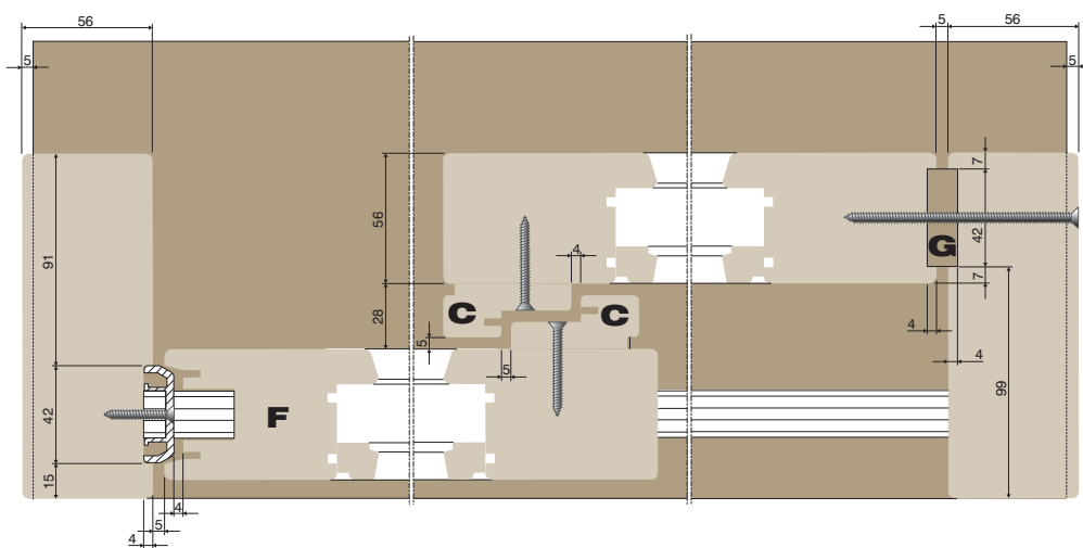
DRAWING BASED ON 68MM SASH
