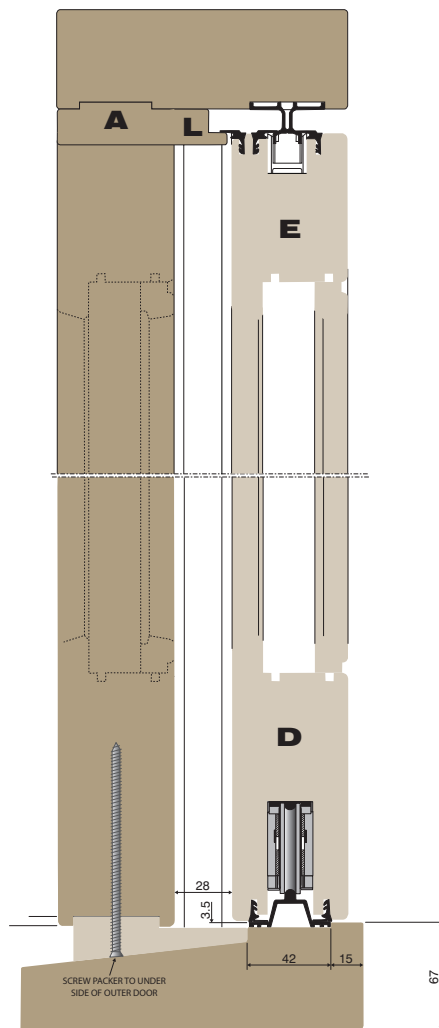
DRAWING BASED ON 68MM SASH
